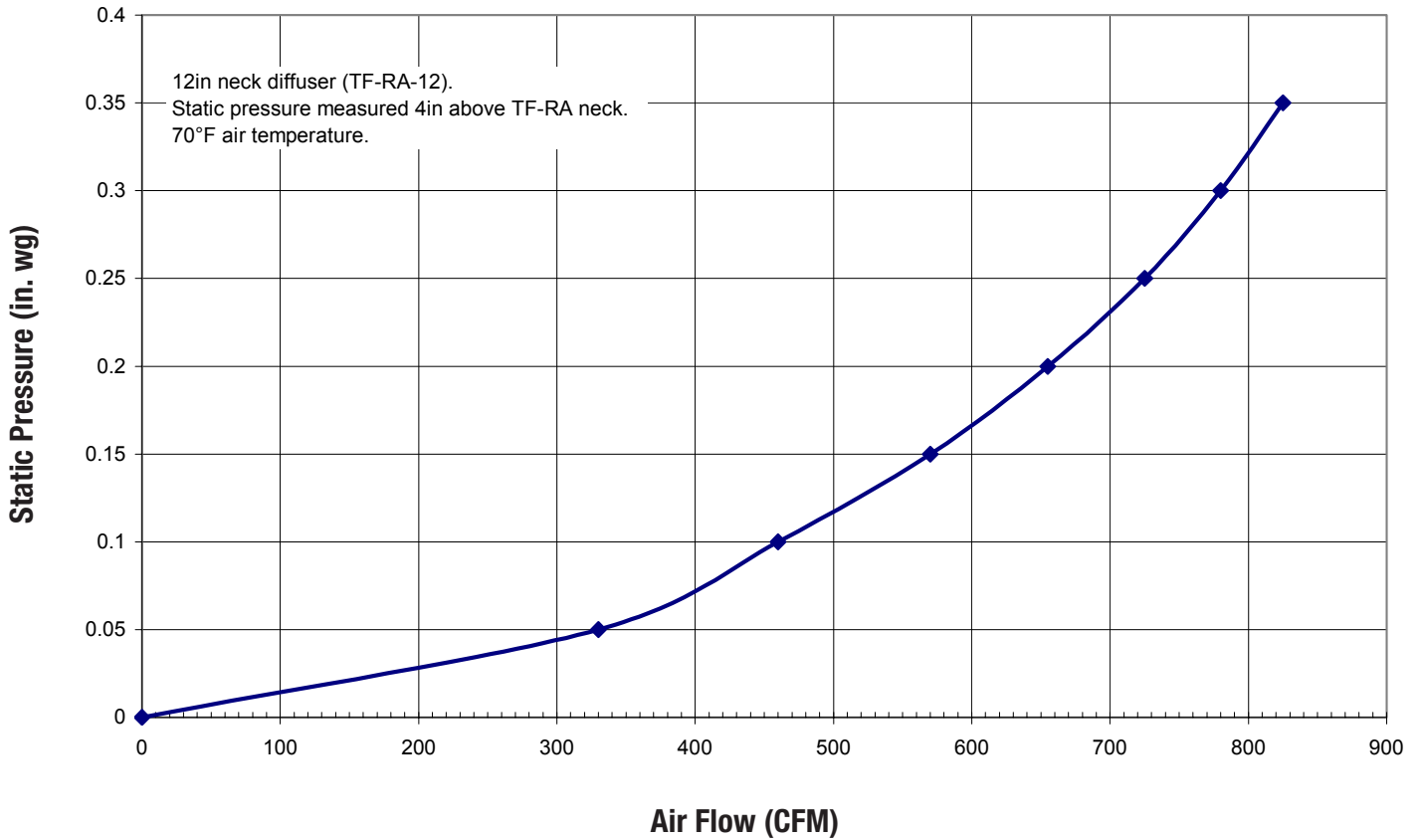
Therma-Fuser Air Diffuser (TF-RA) Performance Pressure Drop vs Air Volume
