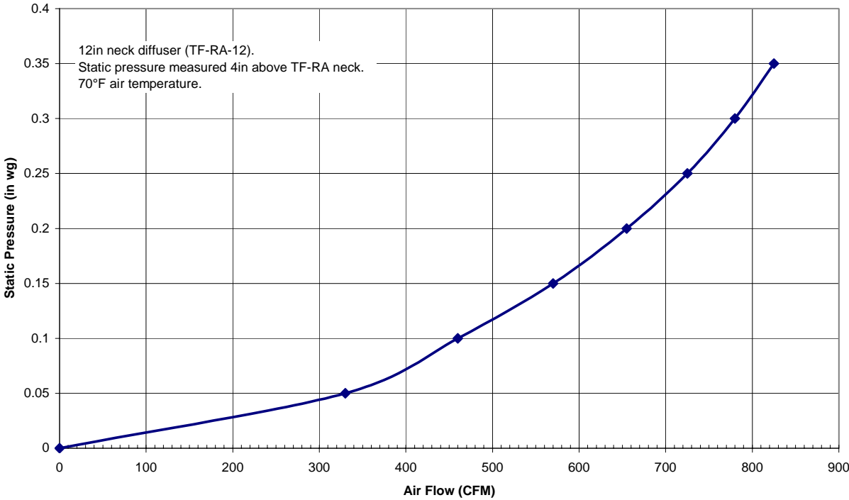
Therma-Fuser Return Air Diffuser (TF-RA) Performance Pressure Drop vs Air Volume
